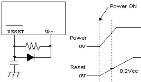
Fig-1 Reset Circuit
