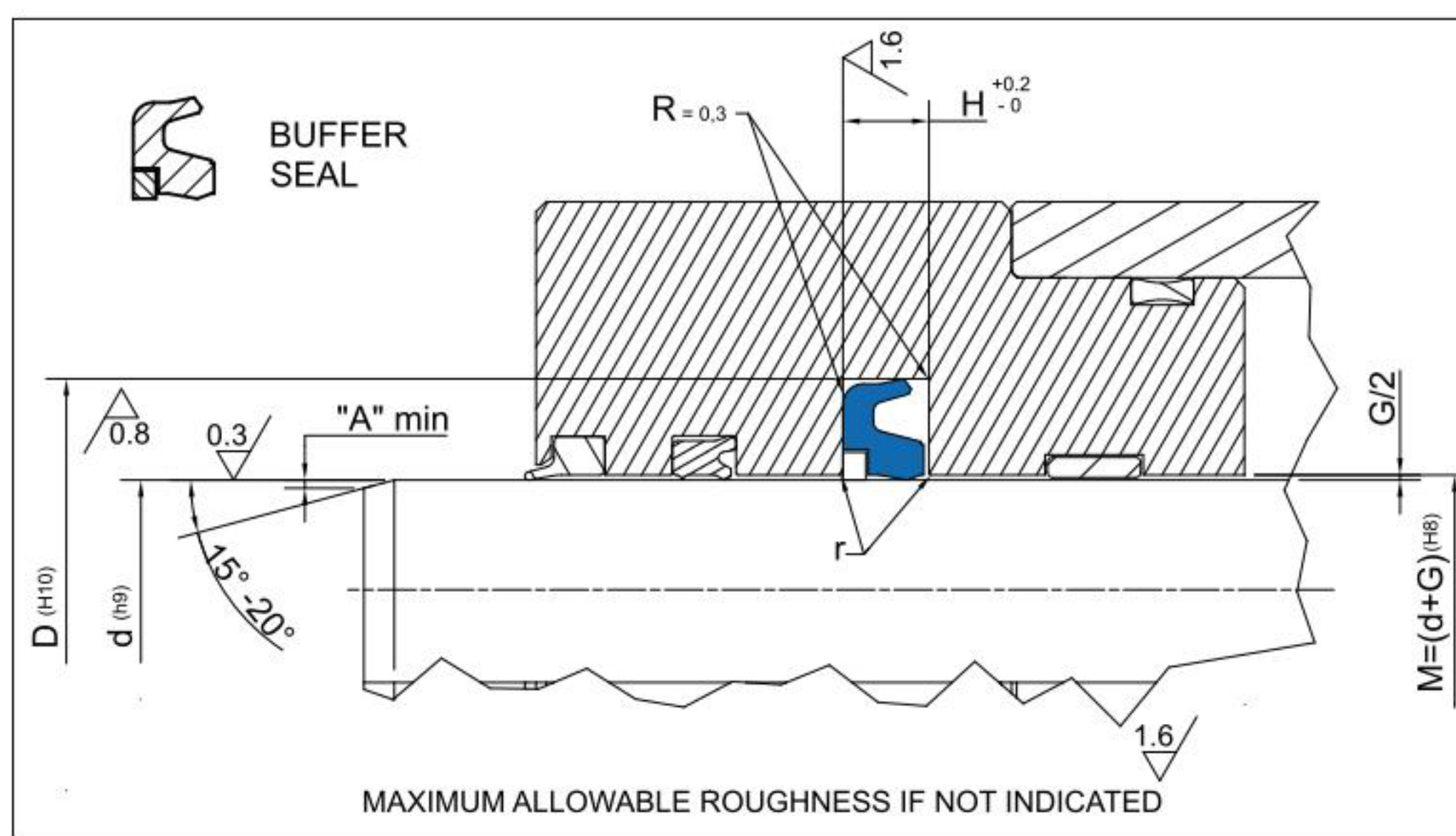
Rod Seal design guidelines
