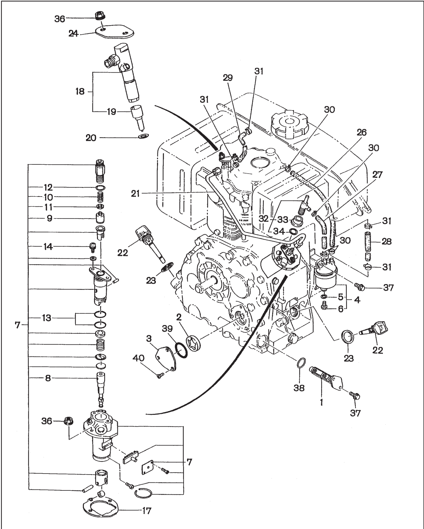
FIG. 10 FUEL SYSTEM GROUP- PTD206T & PTD306
