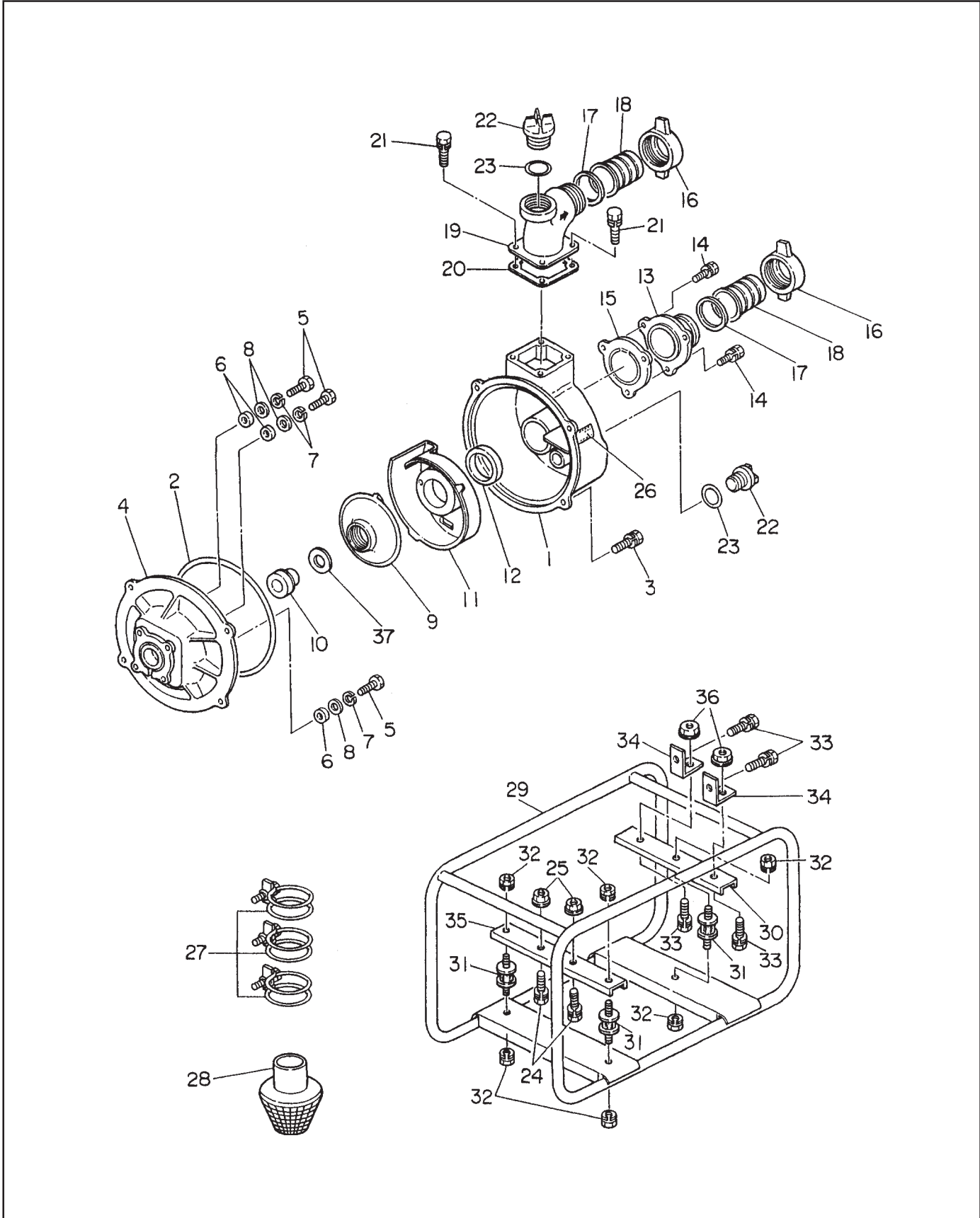
FIG. 1B PUMP - PTD306
