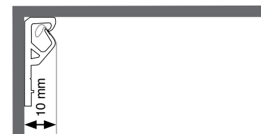
Sketch S10 - DESCOR ® AP profile version
