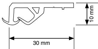
Sketch S06 - DESCOR ® AP profile
