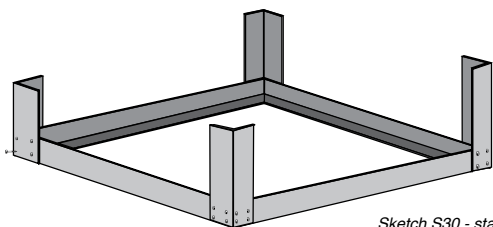
Sketch S30 - standard inspection cover 60 x 60 cm
