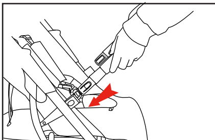
6. As indicated by the arrows, Insert the front bumper into the slot, hear "click" means OK.
