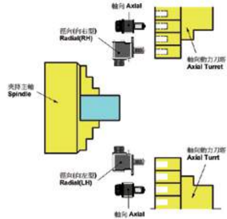
Axial Turret
