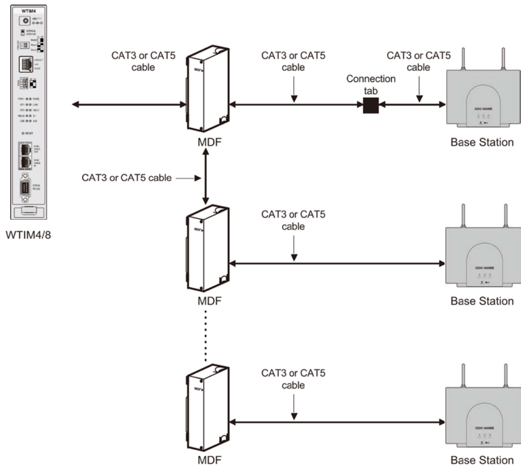
Figure 3.7-3 Wiring with MDF and connection tab between WTIM4/8 and Base Station
