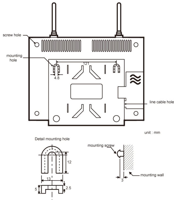
Figure 3.6.2.1-1 Back side of the GDC-600BE
