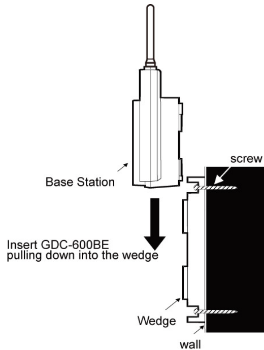
Figure 3.6.2.2-1 Side of GDC-600BE
