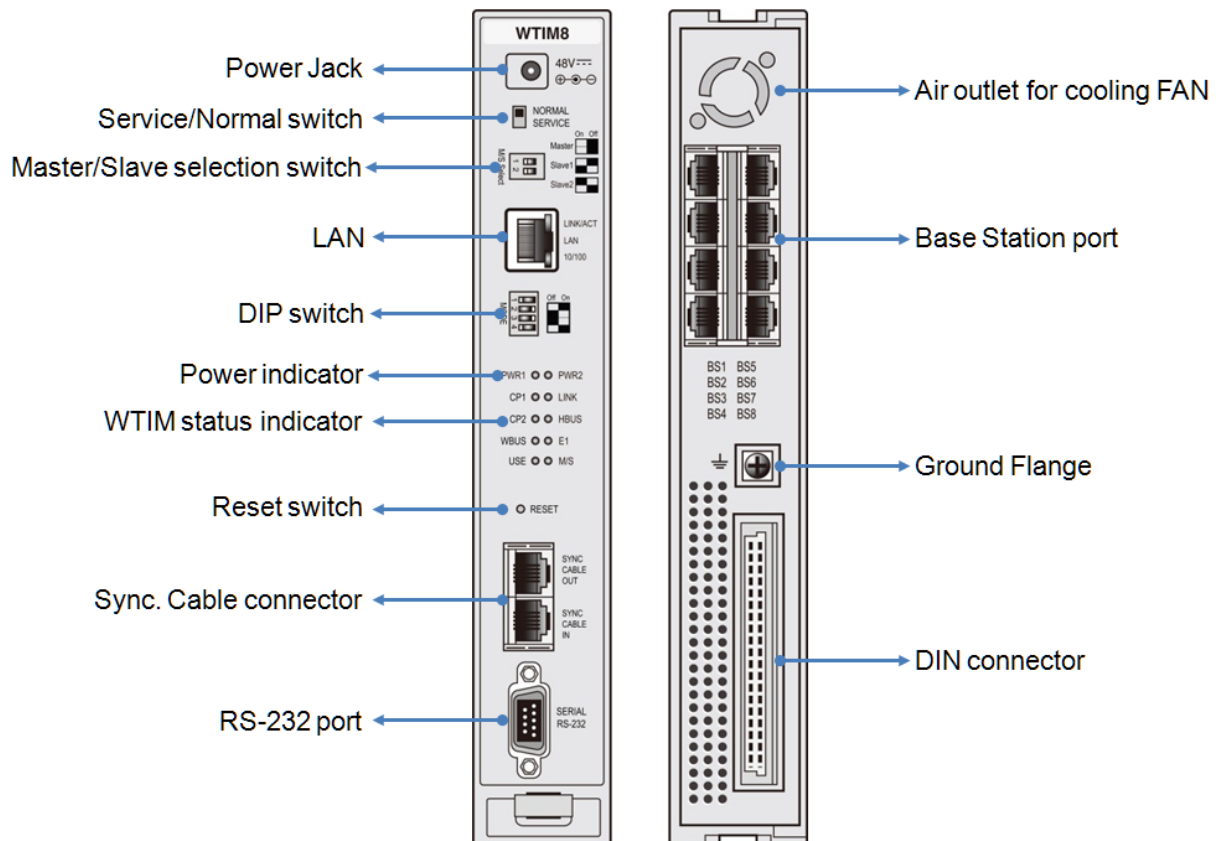
Figure 3.4-1 WTIM8 Front & Rear Panels
