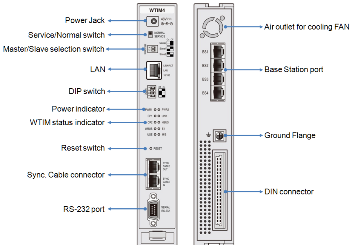
Figure 3.3-1 WTIM4 Front & Rear Panels
