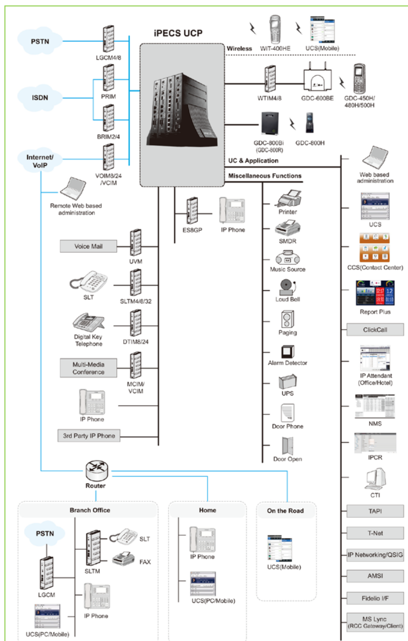
Figure 1.1-1 System Connection Diagram
