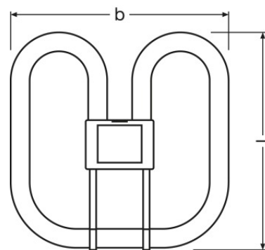
CFL SQUARE 28 W/835 GR10Q, CFL SQUARE 38 W/835 GR10Q
