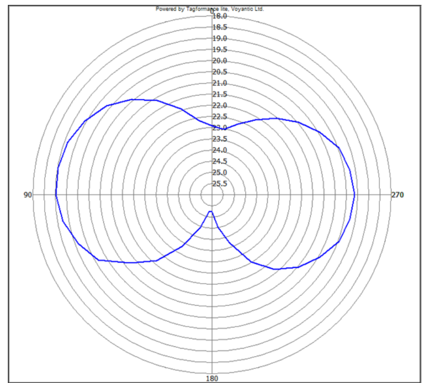
Angular Sensitivity (Relative Read Range vs. Orientation)
