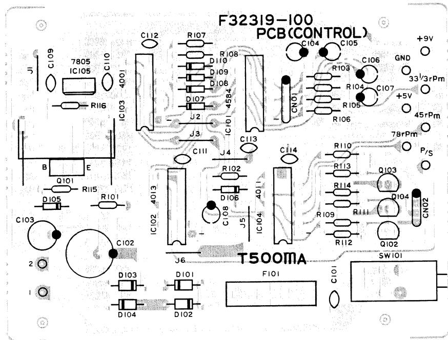
52-1 Control PCB
