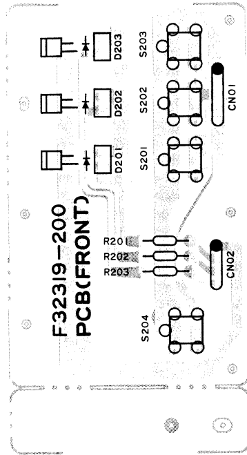
53-1 Front PCB
