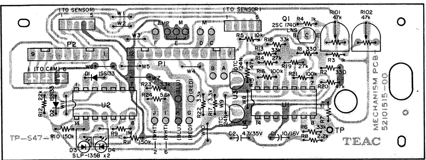
MECHANISM PCB ASSY (R-999X/R-777X)
