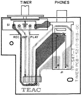
TIMER PCB ASSY (R-999X/R-777X)
