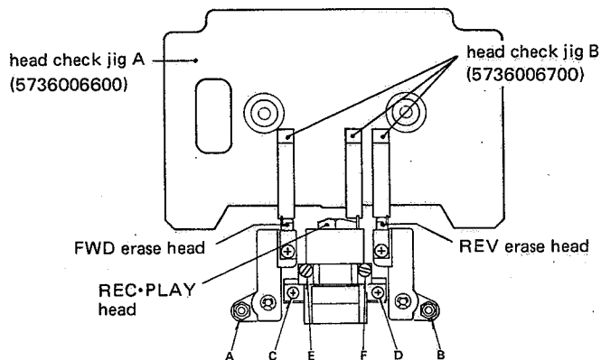
Fig. 4-4 Head height adjustment
