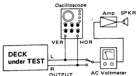
Fig. 4-3 Test setup for azimuth adjustment アジマス調整接続
