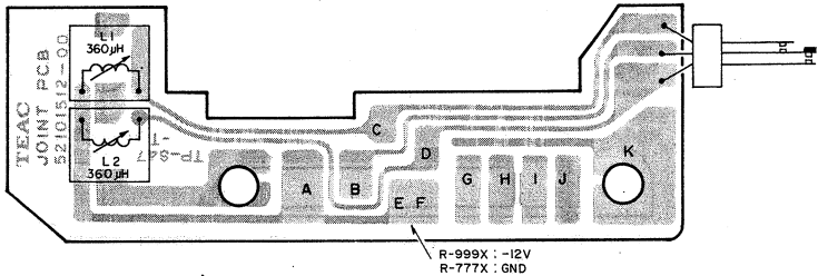
JOINT PCB ASSY (R-999X/R-777X)
