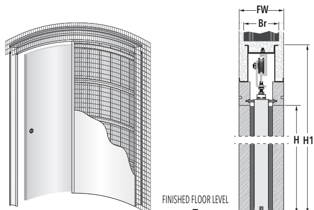
SYSTEMS FOR CURVED DOOR - Measures related to Italian standards, other dimensions available
