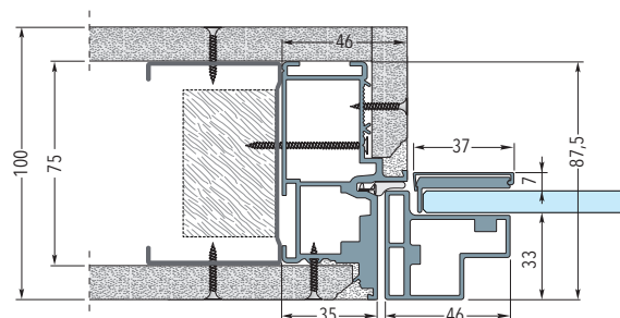
Frame on stud wall with two plasterboards - Finished wall thickness 100 mm
