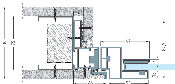
Frame on stud wall with two plasterboards - Finished wall thickness 100 mm
