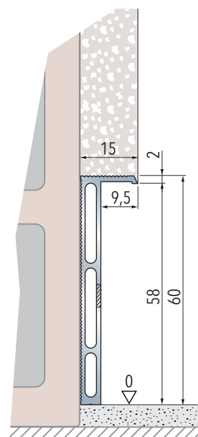
Baseboard installed on solid wall
