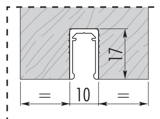
Detail of the door panel with anti-warp profile
