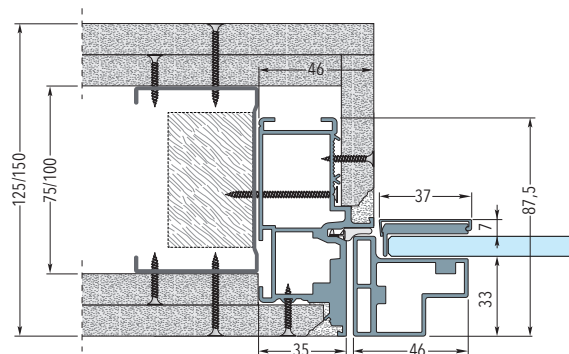
Frame on stud wall with two plasterboards - Finished wall thickness 125/150 mm
