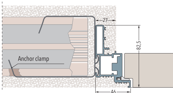
Frame on stud wall with one plasterboard - Finished wall thickness 100 mm
