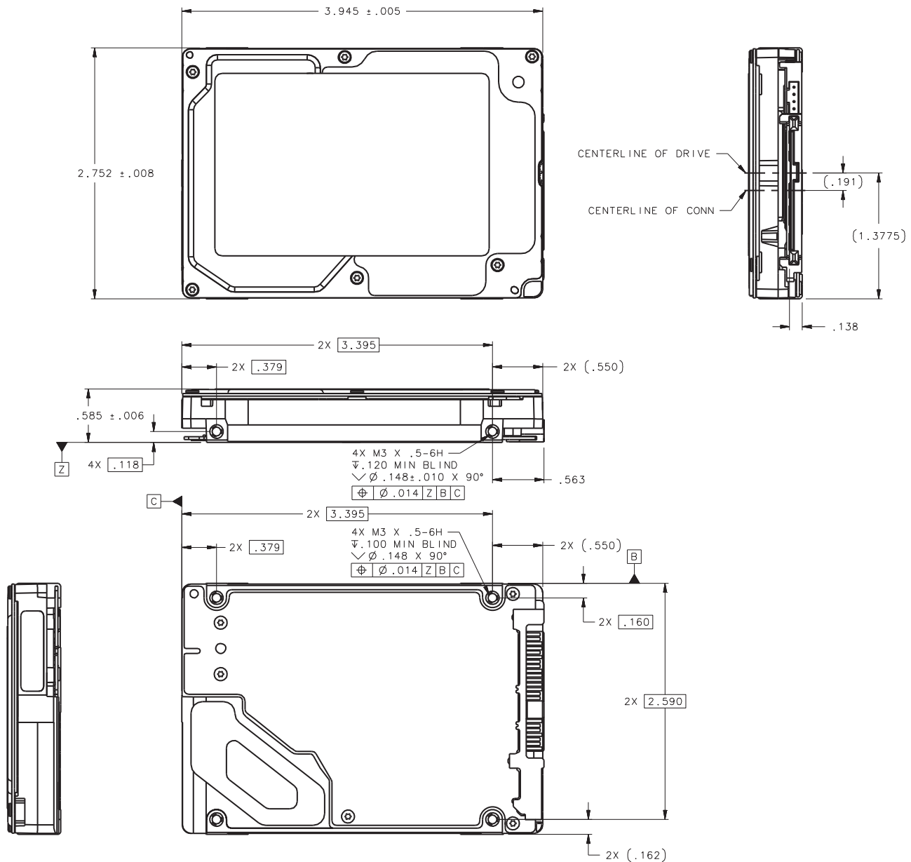
Figure 9. Dimensions
