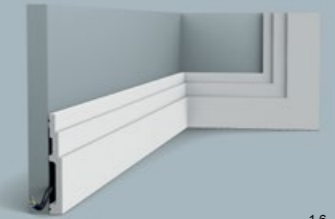
SX180 | SX180F HIGH LINE 200 x 12 x 1,6 cm Duropolymer®
