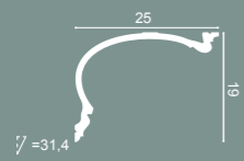
C343 HERITAGE XL 200 x 19 x 25 cm Purotouch®
