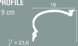
C343 HERITAGE XL CURTAIN PROFILE 200 x 19 x 25 cm Purotouch ®
