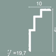
C392 STEPS 200 x 19 x 10 cm Purotouch ® Designed by Orio Tonini
