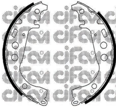
153-431 (Ø 203,0 x 32)
