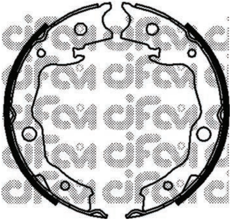
153-295 (Ø 172,0 x 32)
