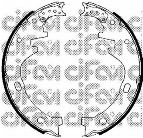
153-274 (Ø 254,0 x 46)
