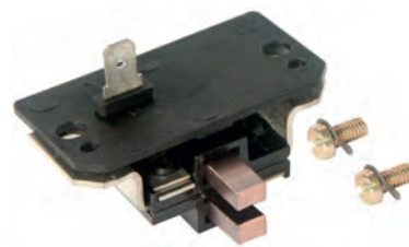
131704 Brush Box
