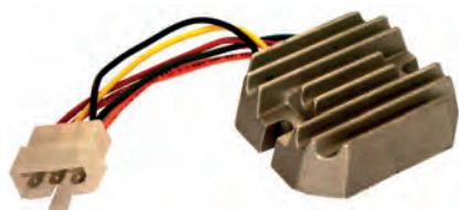
234412 Regulator/Rectifier Replacing: RS5160 14 Volt, 20 Amp, Dist. mount. holes 63.55 20 A charging system. Terminals: B+(red), IG(yellow), B-(black), AC(orange), L(brown), AC(orange).
