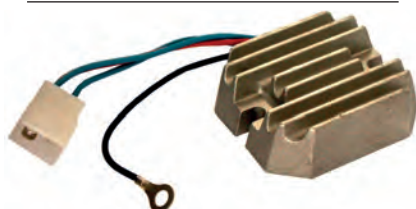
234410 Regulator/Rectifier Replacing: RS5107 14 Volt, Dist. mount. holes 63.00
