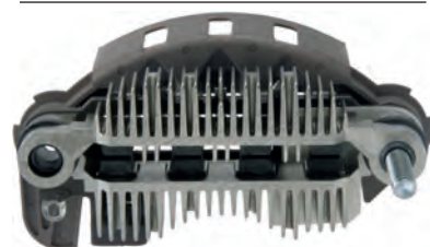
236559 Rectifier Replacing: RM-154HV, 31127-PGM-004 Servicing: 31100-PND-004, A002TB7591, A002TB8691, A002TC0691, A002TC0691A, A002TC0691AE, A002TC0691ZE, A2TB7591, A2TB7951 B+ M6, B+/threaded M6/24.53, ID 28.00, OD 99.00, Mount. dist. 85.00, B+ type Bolt, No./diodes 8, Capacitor w/ Alternative no.: 333823
