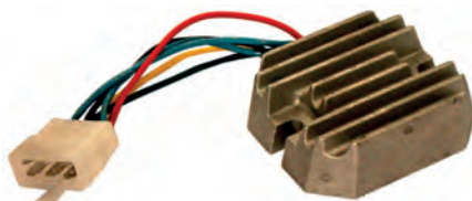
234411 Regulator/Rectifier Replacing: RS5155, RS5101 14 Volt, Dist. mount. holes 62.55, Regulator type Electronic Terminals: AC(blue), B-(black), AC(blue), L(green), B+(red), IG(yellow).
