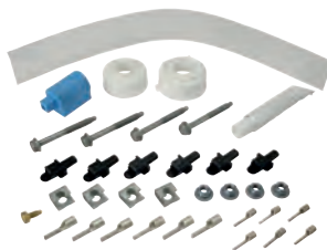
230423 5★ Repair Kit
