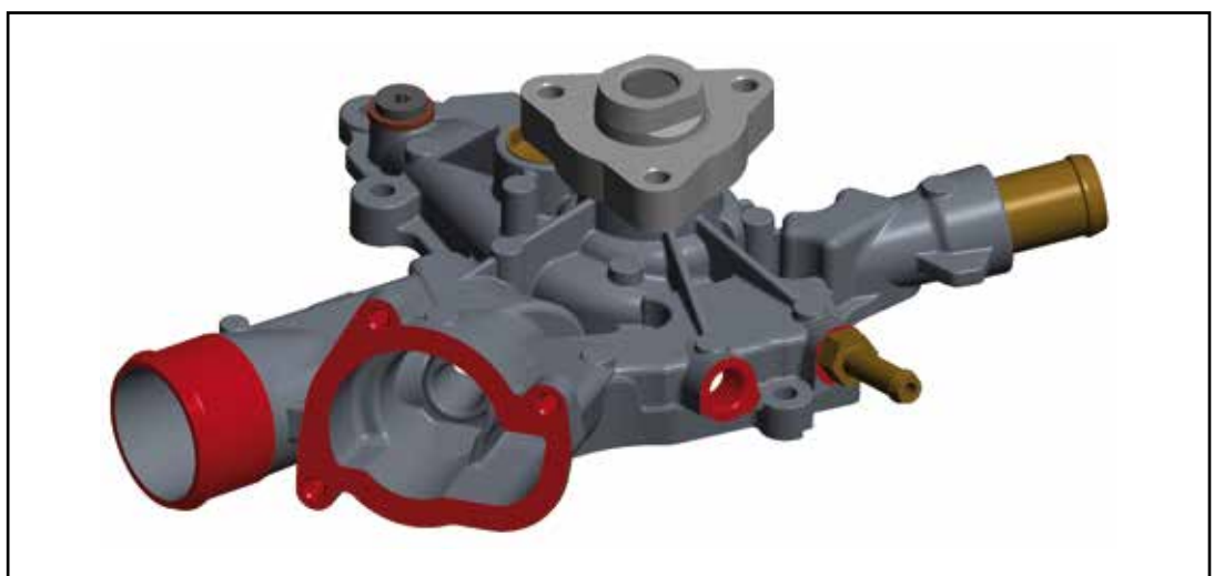
2.1 Water Pump with integrated thermostat housing
