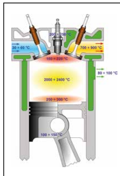
1.1 Temperatures in the various areas of the engine
