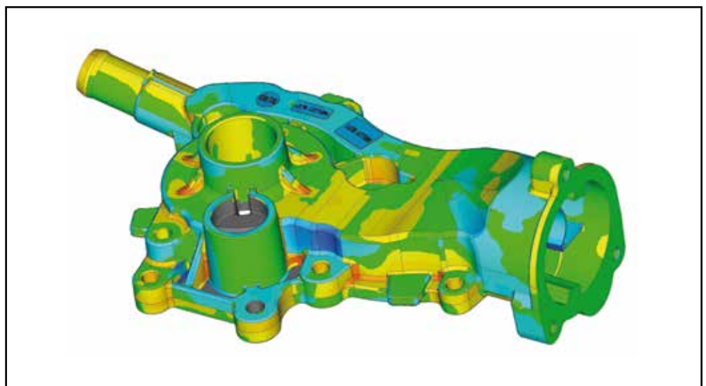
5.2 3D dimensional control water pump housing
