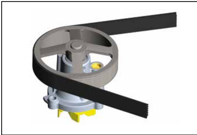
3.3 Water pump with a Poly-V power take off
