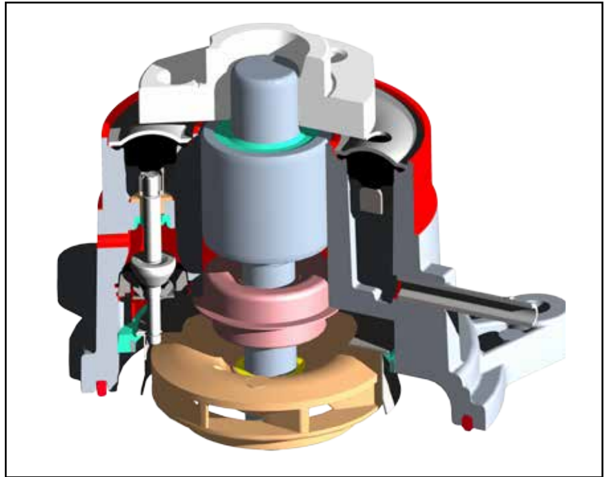
12.1 Section of the switchable water pump patented by Metelli
