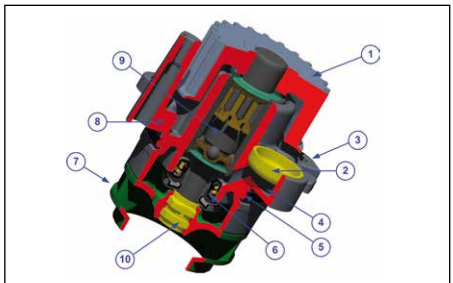
4.1 Section of a water pump and its components
