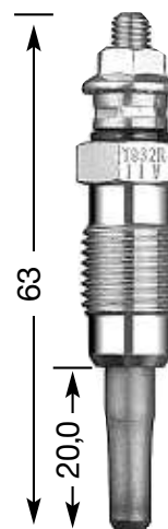
Y-932 R M 12 x 1.25 12 Hex 11 V
