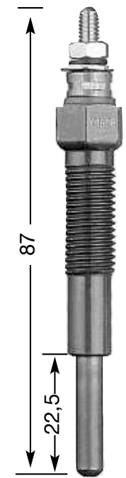
Y-157 R M 10 x 1.25 12 Hex 23 V
