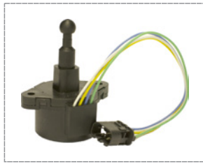
Leveling Motor 20-0011-MA-1 RH=LH 67168372381
