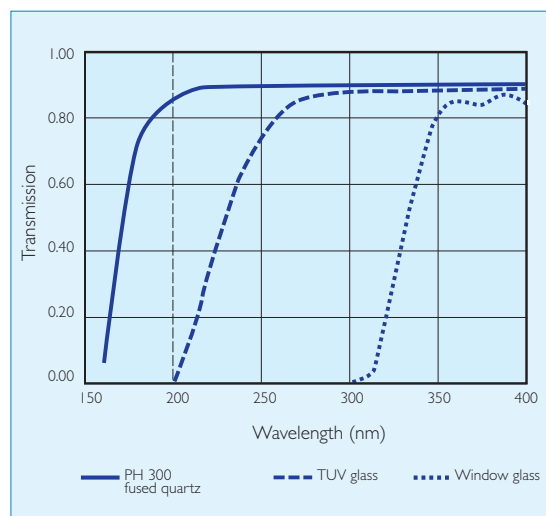
■ Fig 11. Special transmission of glasses (1mm).
