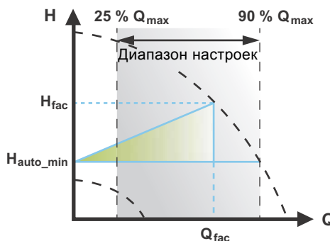
Рис. 35 FLOW_{ADAPT}
