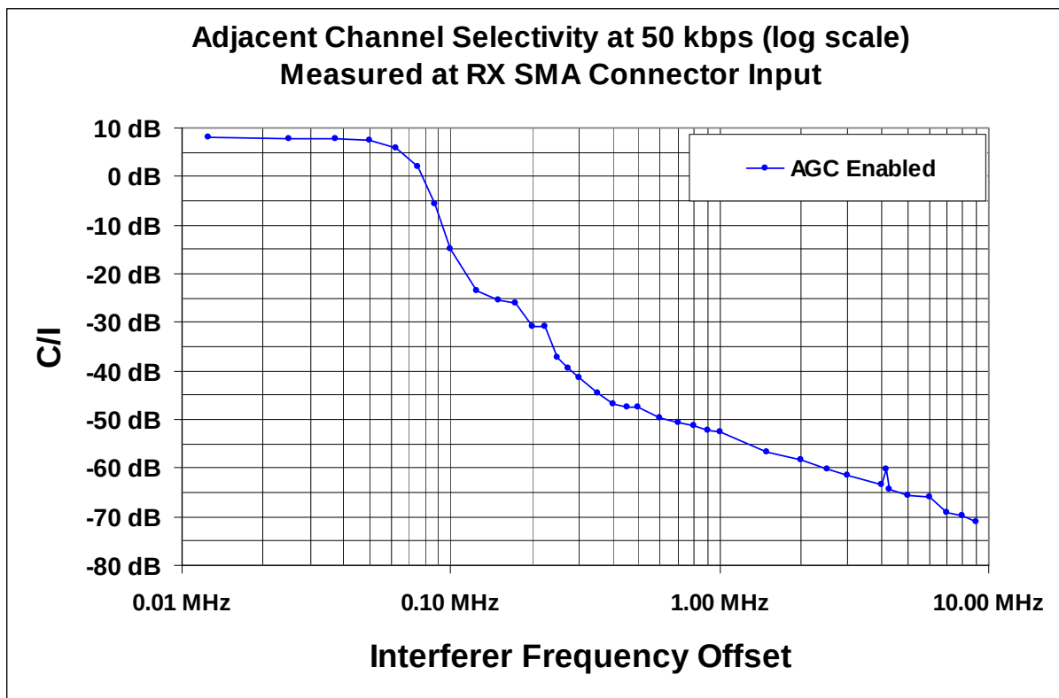
Figure 45. Receiver Selectivity
