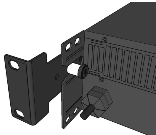
Figure 3.2c: Use tube for slide-on installation.
