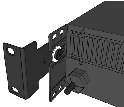
Figure 3.2b: Use washer for fixed installation
