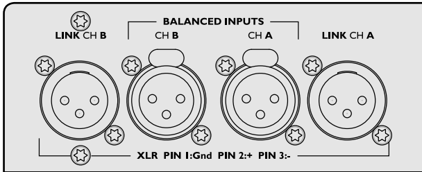
Figure 5.4.1a: Audio inputs and loop-thru
