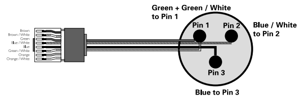
Figure 5.7.2: NomadLink RJ45 to XLR wiring schematic
