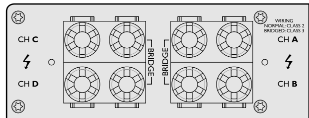
Figure 5.4.4b: Binding Post outputs -
