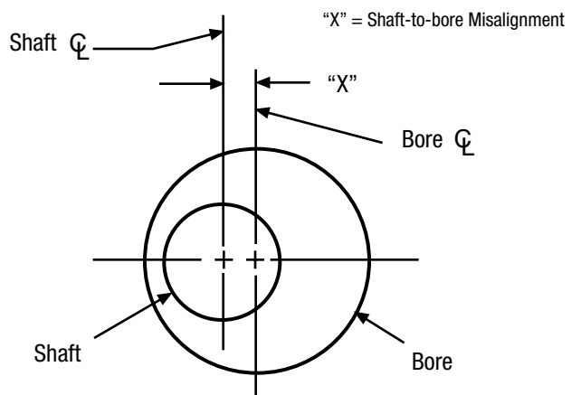
Figure 5 — Shaft-to-bore Misalignment
