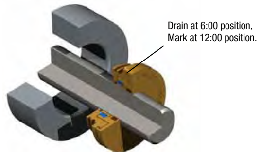
Figure 21 — Drain Port Positioning
