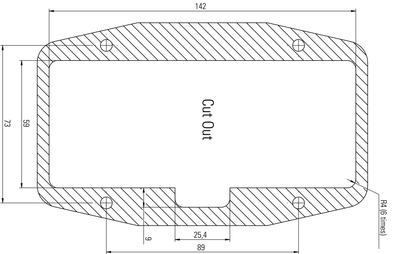
FIG. 10 SINGLE CONTROL LEVER "TEMPLATE"
