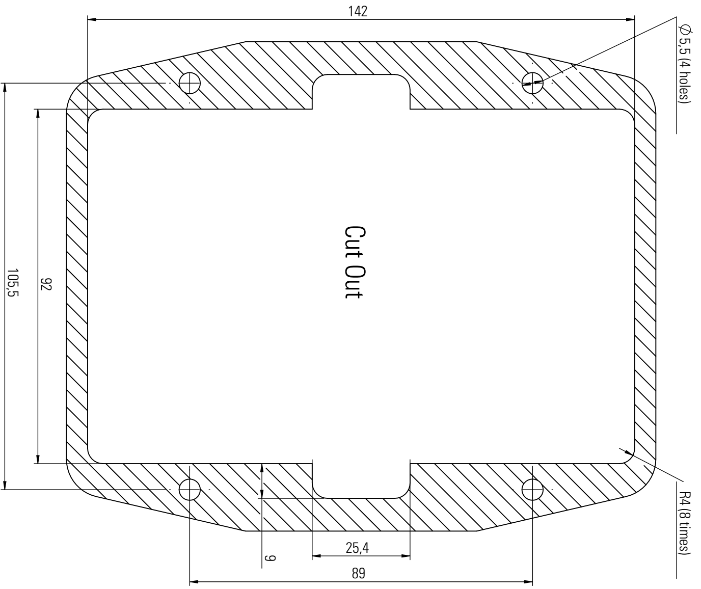
FIG. 9 DOUBLE CONTROL LEVER "TEMPLATE"
