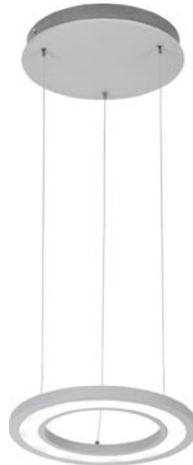
6387 ↑ 68 cm Ø 29 cm 18W ~230V, 50Hz 4000 K, 1800lm
