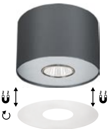
6003 POINT SILVER / GRAPHITE S ↑ 8 cm ∅ 13 cm 1 x GU10 max 35W
