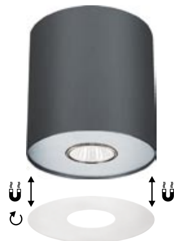
6004 POINT SILVER / GRAPHITE M ↑ 13 cm ∅ 13 cm 1 x GU10 max 35W
