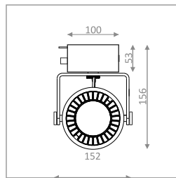
A PHIL53 SK LED VIGO LED ceiling • strop 1800 lm; 23 W
