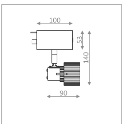
PHIL 53 SK LED MAXI STAR TECHNO GU10; 230 V; 50 W
