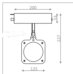
A PHIL53 SK LED TOMA LED; 2700 lm; 34 W
