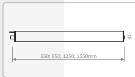
GREY SK connector Z - 74760020 anod.
