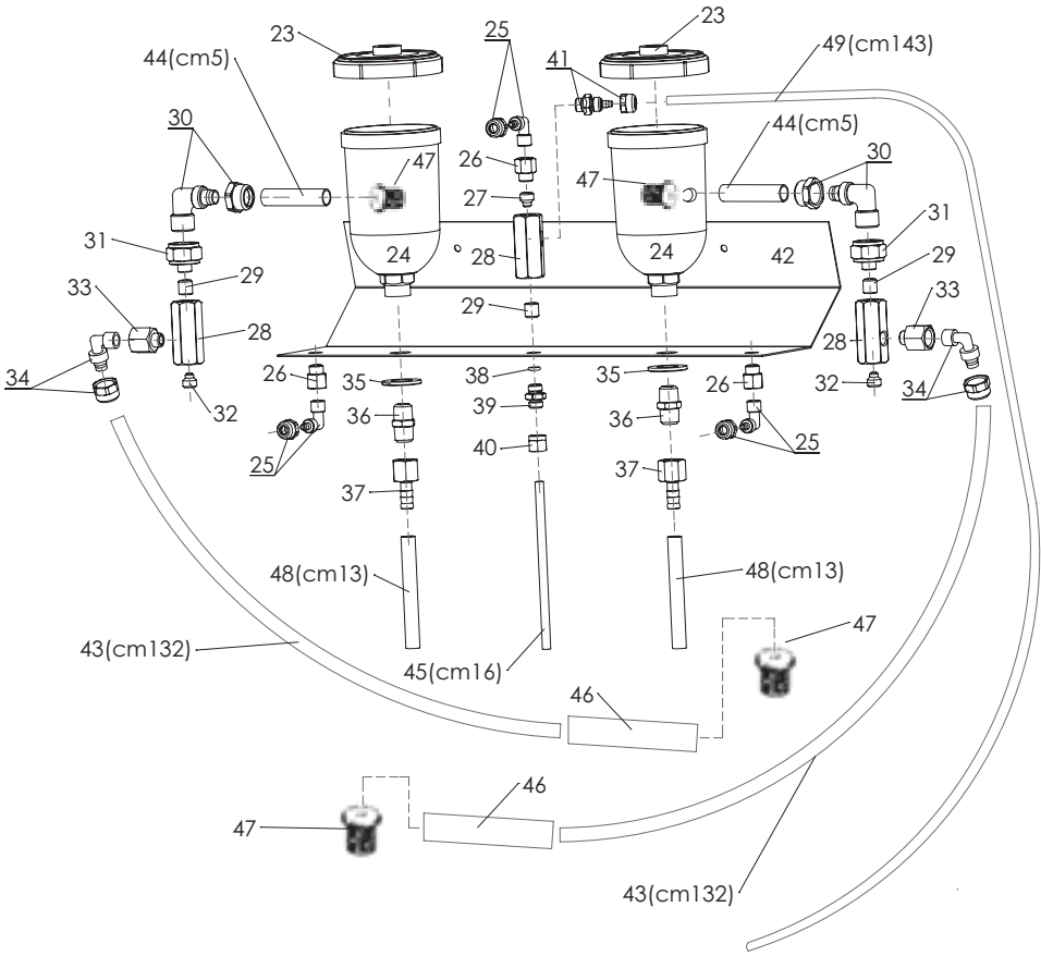
NOZZLES SUPPORT ref. A030018
