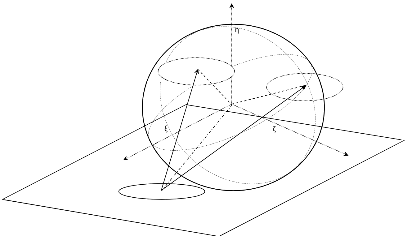
Picture 0.003. Gravitation potential point transduction (gamma radiation). Sky sphere 3D view
