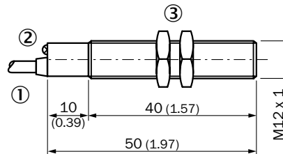
MM12-60A-N-xUx, M12, cable
