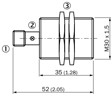
IME30-xxBxxxC0K, flush, connector, short-body housing
