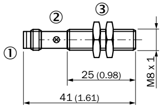
IME08-xBxxxxTOK, flush, connector, short-body housing
