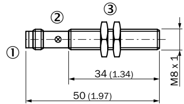
IME08-xBxxxxTOS, flush, connector, standard
