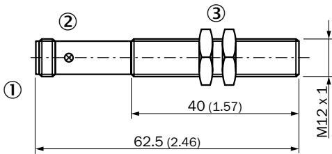
MM12-60A-N-xCx, M12, connector
