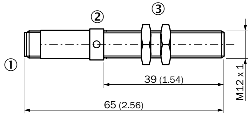
IMF12-xxBxxxxxx, M12, flush
